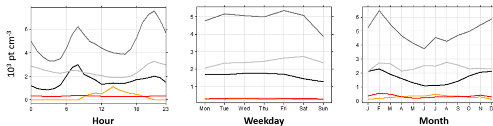
Fig. 3. Daily, weekly and monthly patterns of the sources identified in each city. In Barcelona, Traffic 1 and Traffic Nucleation sources are all included as Traffic Nucleation .
